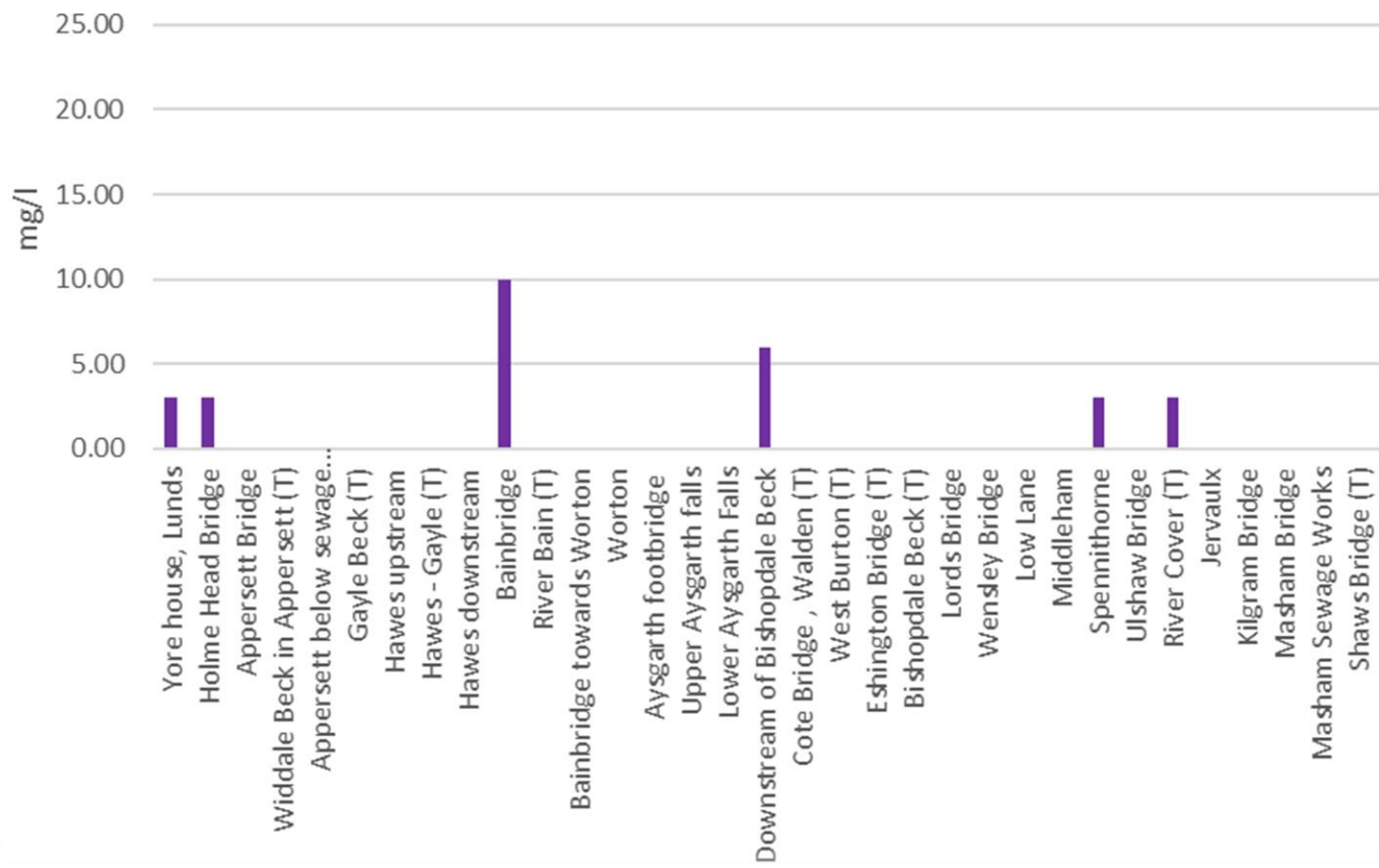
River Ure Sampling 21.8.24 - Suspended Solids
