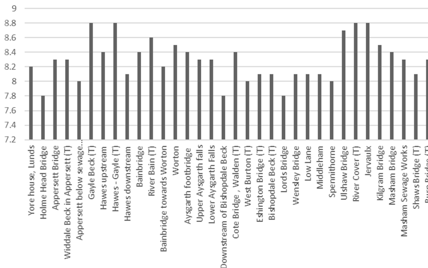
River Ure Sampling 21.8.24 - pH
