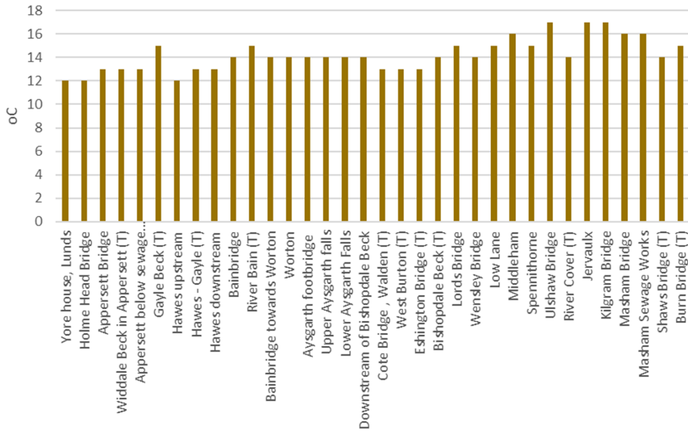
River Ure Sampling 21.8.24 - Temperature
